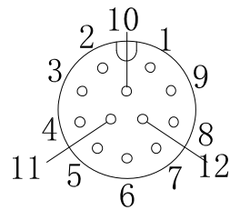
Pin Assignment Front View
