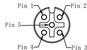
Pin Assignment Front View Female
