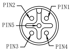
Pin Assignment Front View Male
