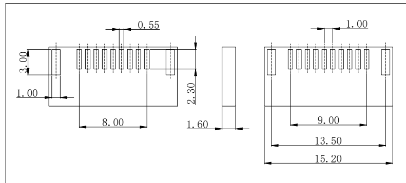
REFERENCE PCB LAYOUT
