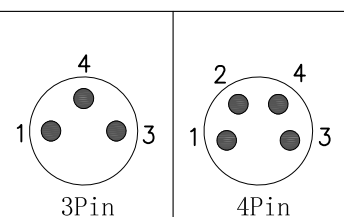
Pin Assingments Front View
