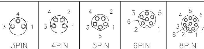
Pin Assingments Front View
