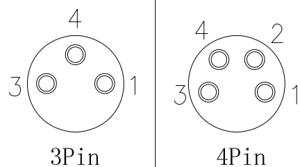
Pin Assignment Front View
