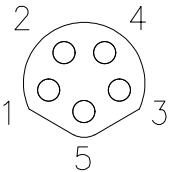
Pin Assingments
