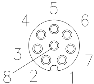
Pin Assignments
