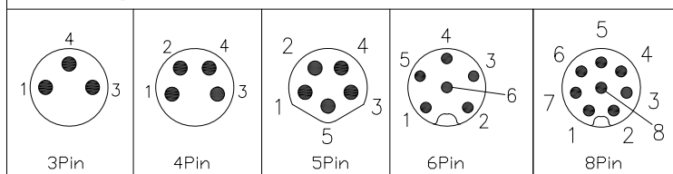
Pin Assignments Front View
