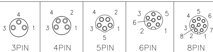
Pin Assingments Front View
